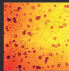
Photomicrograph showing graphite form in ductile iron.
